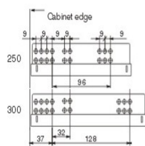
Drawer size and boring
