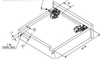
Drawer size and boring
